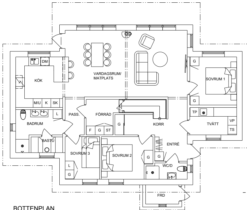
BOTTENPLAN
